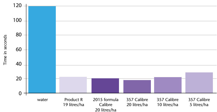
Droplet Penetration Test Average of 20 results
